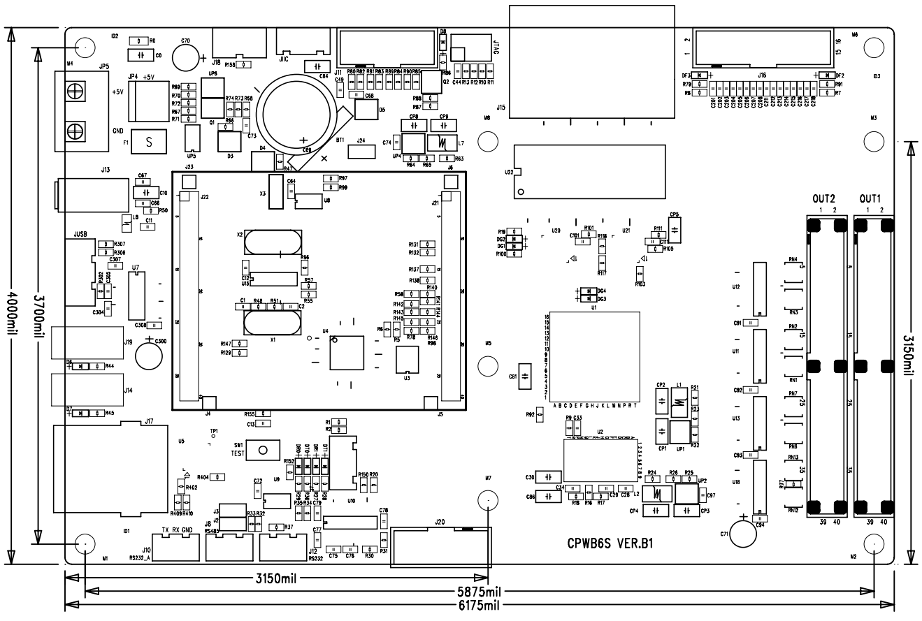
CPWB6S VER.B1 SILKSCREEN TOP
