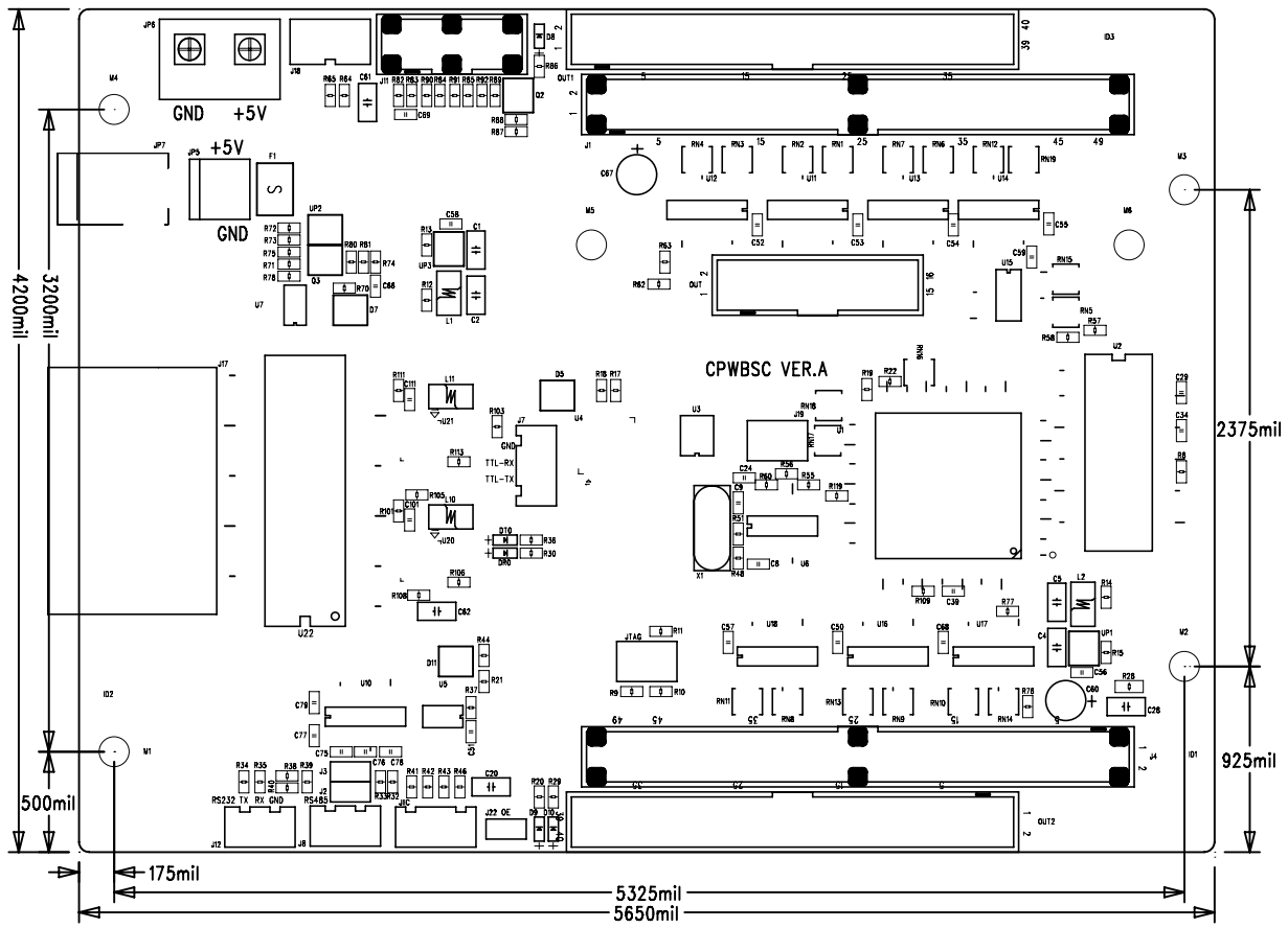
CPWBSC VER.1 SILKSCREEN TOP
